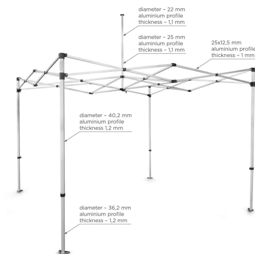
Aluminium profiles: legs 40.2 / 36.2 mm, roof arms 25 x 12.5 mm, mast 25 / 22 mm
